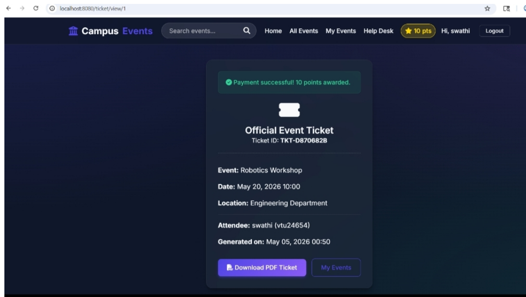
Figure 5.4: Event Registered
